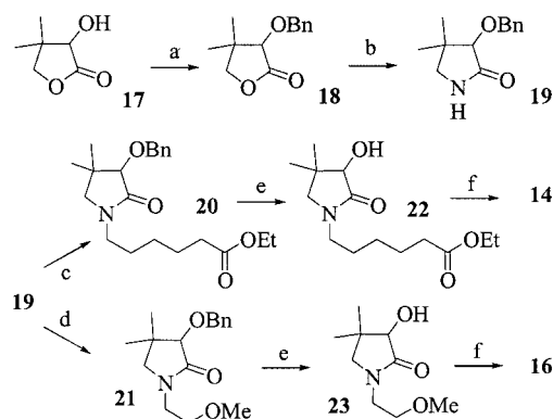
Scheme 2. Reagents: (a) BnBr, \text{Cs}_2\text{CO}_3 , DMF; (b) \text{NH}_3 aq., 230 °C; (c) NaH, \text{Br}(\text{CH}_2)_5\text{CO}_2\text{Et} , DMF; (d) NaH, \text{Br}(\text{CH}_2)_2\text{OMe} , DMF; (e) \text{H}_2 , \text{Pd}(\text{OH})_2 , EtOAc; (f) acryloyl chloride, \text{NEt}_3 , \text{CH}_2\text{Cl}_2
