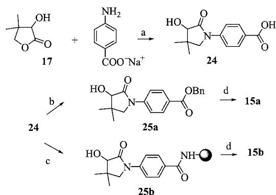
Scheme 3. Reagents: (a) 190 °C, 72 h; (b) BnOH, BOP/DIEA, DMF; (c) polymer- \text{NH}_2 ; BOP/DIEA, DMF; (d) acryloyl chloride, \text{NEt}_3 , \text{CH}_2\text{Cl}_2
